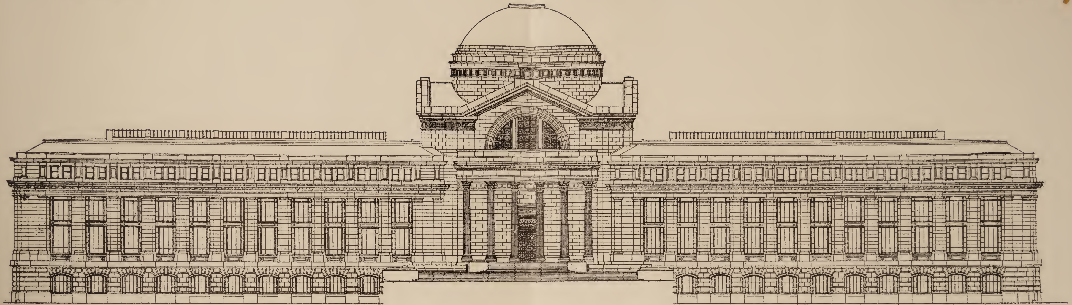
SOUTH ELEVATION OF BUILDING.
